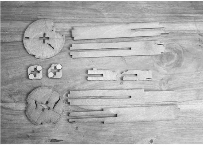
18) Layout of the parts needed to assemble the masts of the ship. Repeat following steps on both the large and small masts.
